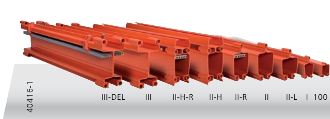
BKK steel profile sections
